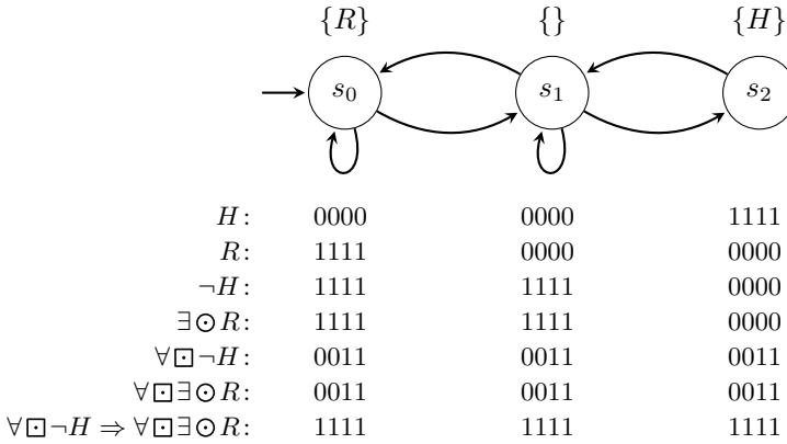
Fig. 1 A Kripke structure that tracks a possible interaction between a robot and office workers. Within each state, we mention its identifier. Above each state, we mention its label. Below each state, we mention the maximal valuation that holds in the state for each subformula of \Phi = \forall \square \neg H \Rightarrow \forall \square \exists \odot R .
