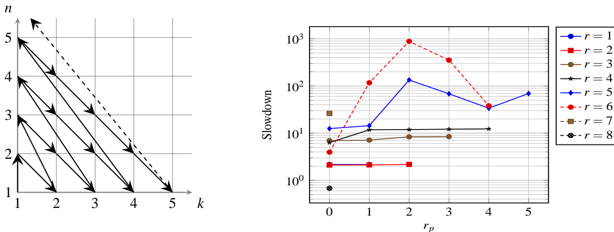
Figure 1: The search strategy for some realizing implementation on the left-hand side and the slowdown of PROMPT-LTL synthesis on the right-hand side.
