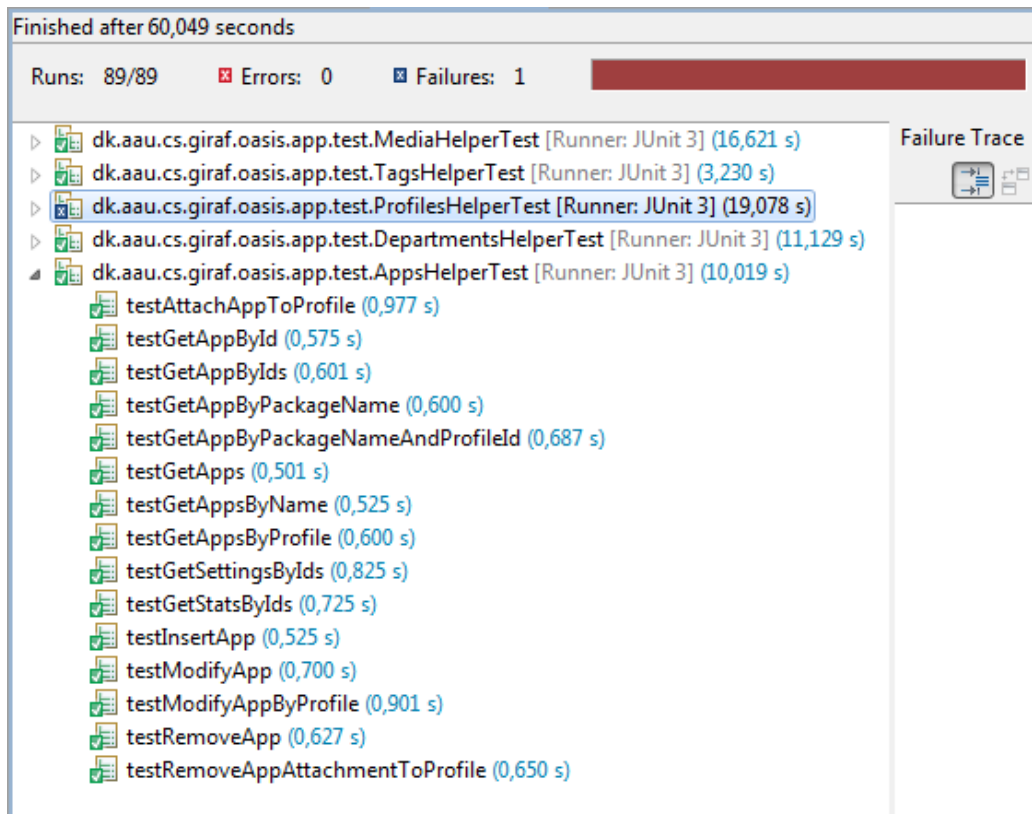
Figure 19.1: The result from the appsHelper tests.
