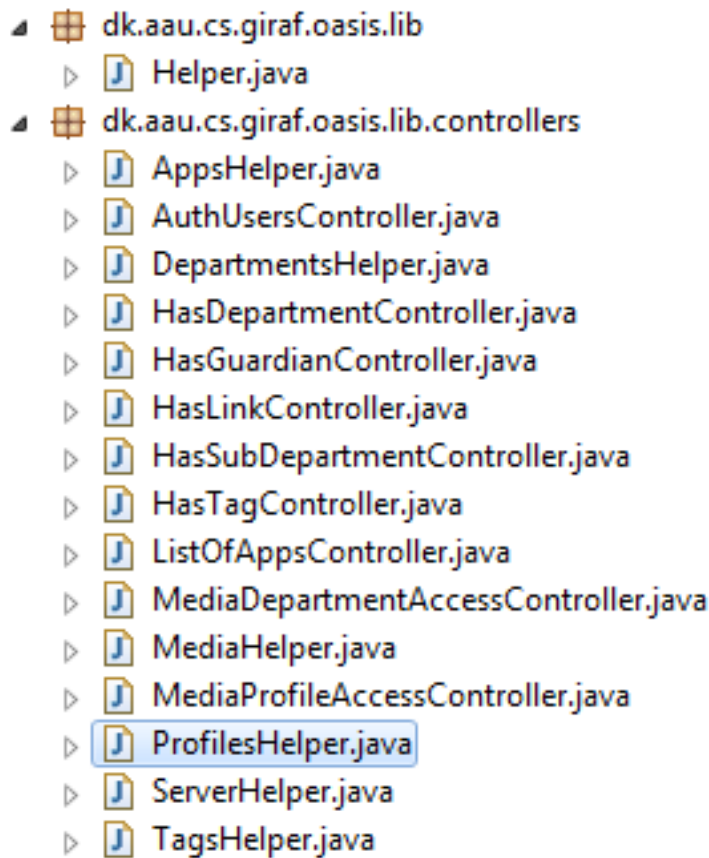
Figure 5.2: The controllers in the Oasis Lib
