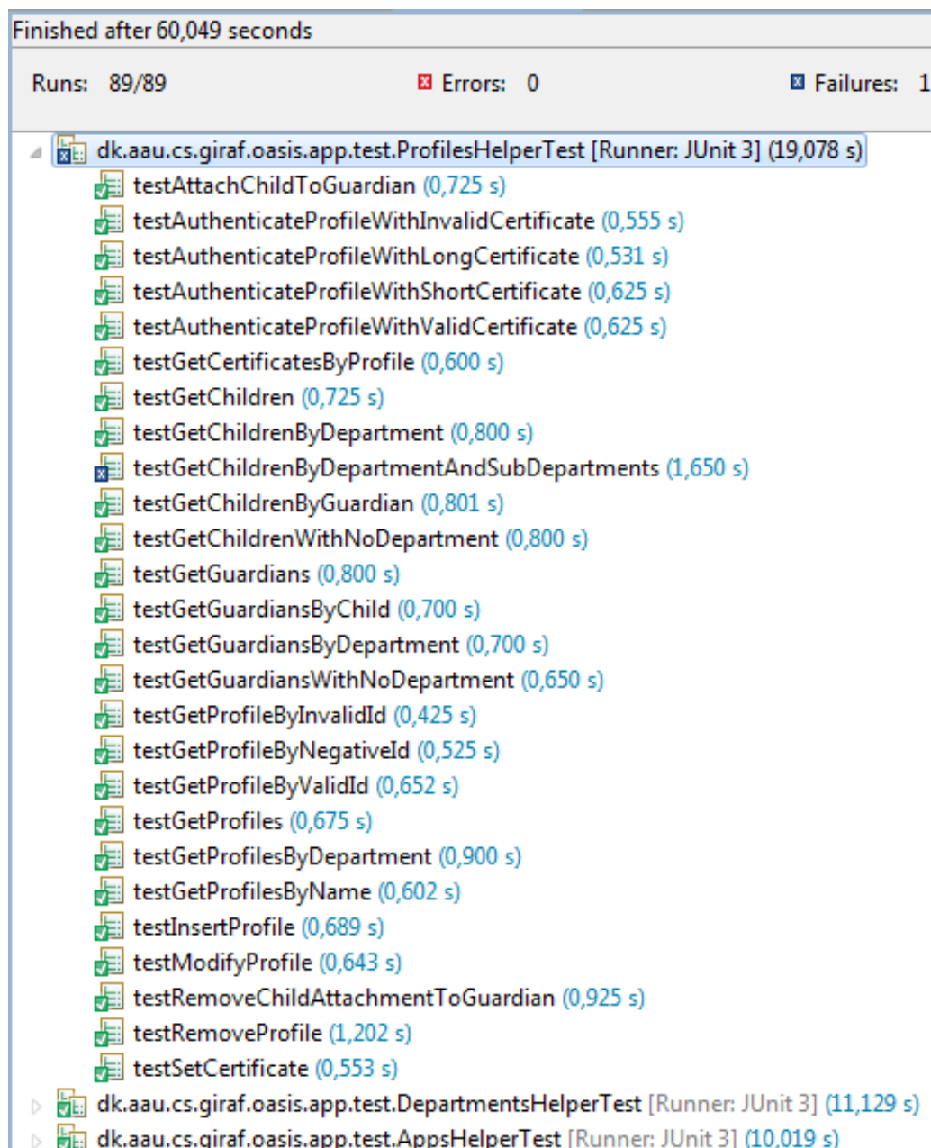
Figure 7.2: The result from the profilesHelper tests.
