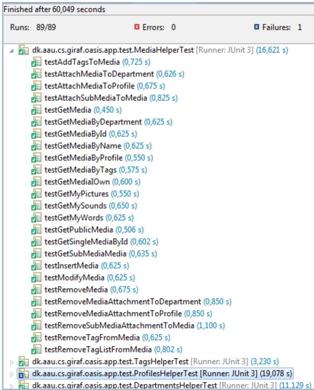
Figure 19.3: The result from the mediaHelper tests.
