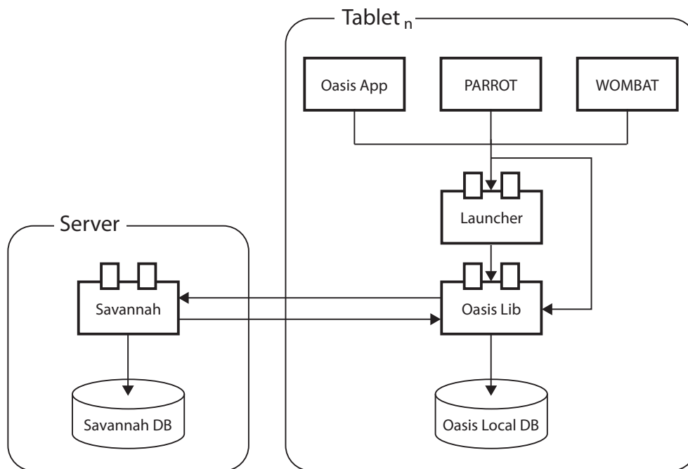
Figure 1.1: The GIRAF architecture
