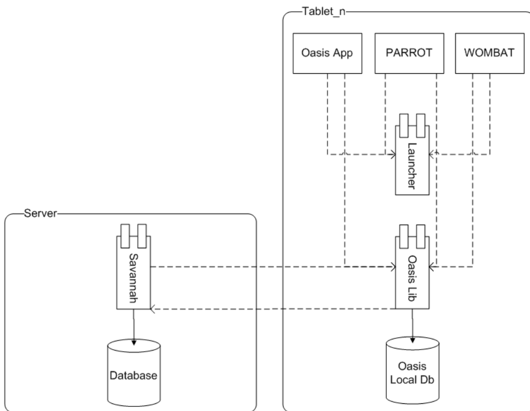
Figure 2.1: The GIRAF system architecture.
