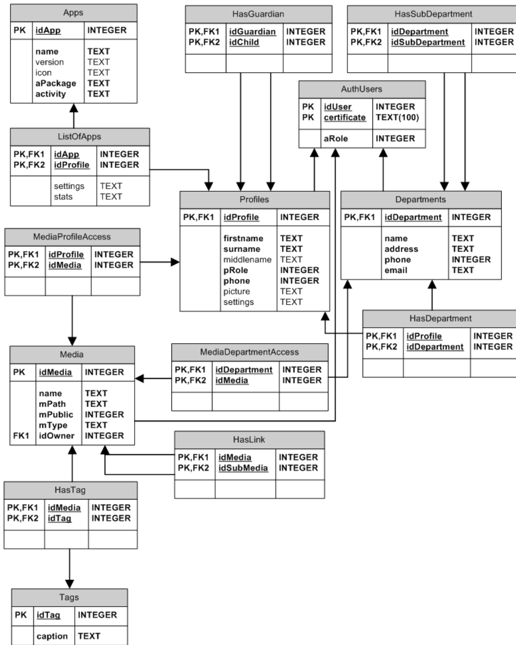
Figure 4.1: The schema for the Oasis Local Db.
