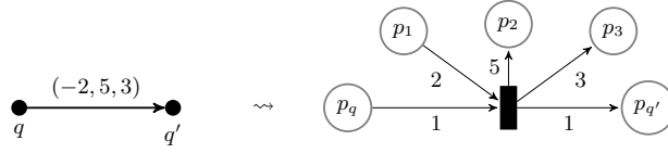
Fig. 3: Translation of a 3-weighted automaton to a Petri net
