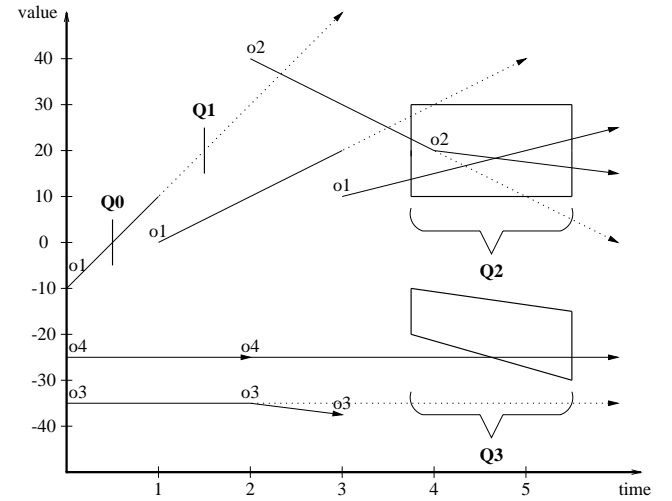
Figure 2: Query Examples for One-Dimensional Data
