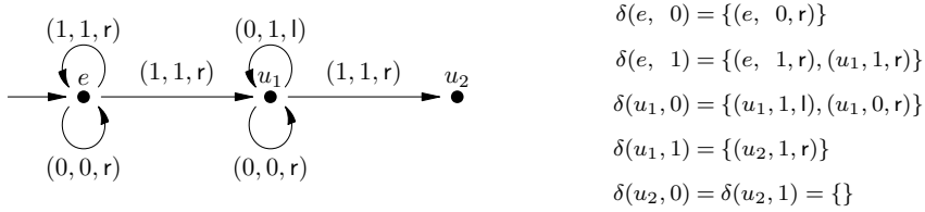
Fig. 1. The transition relation of an ATM as a labelled graph and a function.
