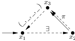
Fig. 5. Specification M_{exist} enforces a \pi -transition after each \exists -transition.
