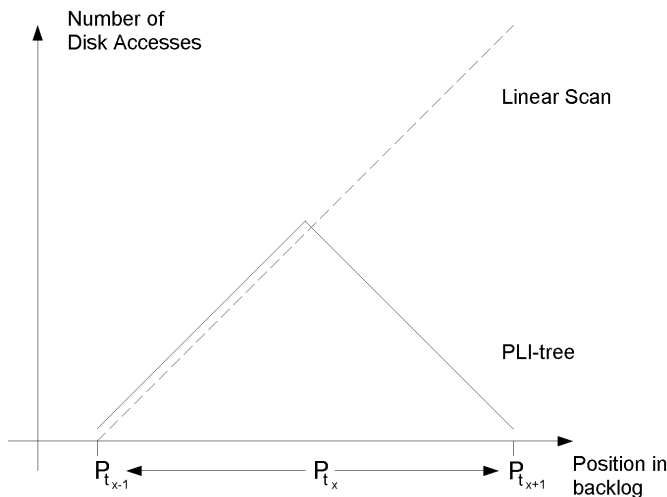
Fig. 8. Cost comparison of timeslice computation using linear scans vs. PLI-trees.
