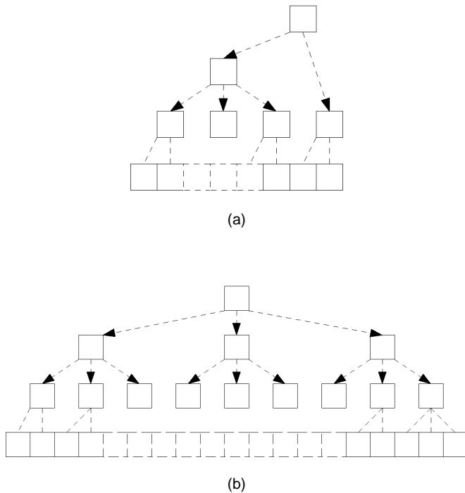
Fig. 9. Situations: (a) worst-case; (b) best-case.
