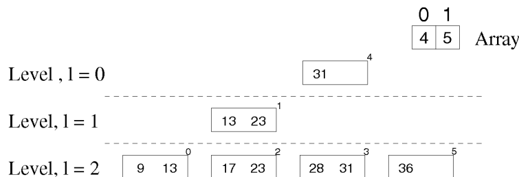
Fig. 4. A PLI-tree of height h = 2 and order d = 3 .
