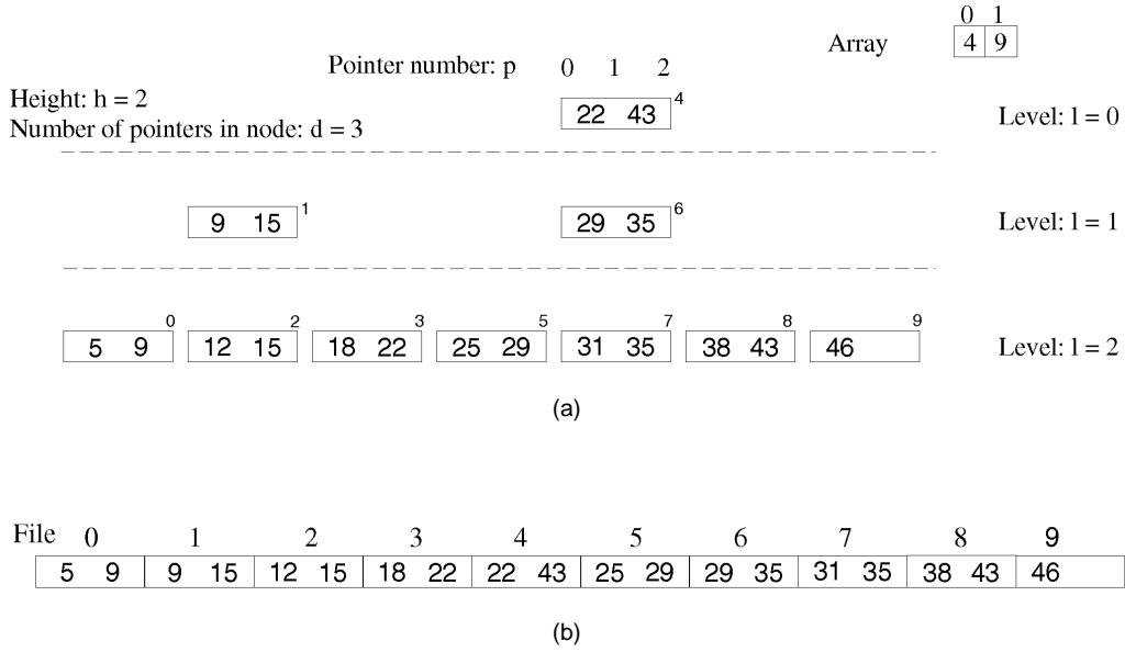
Fig. 5. An example of a PLI-tree and how nodes are stored in a file.
