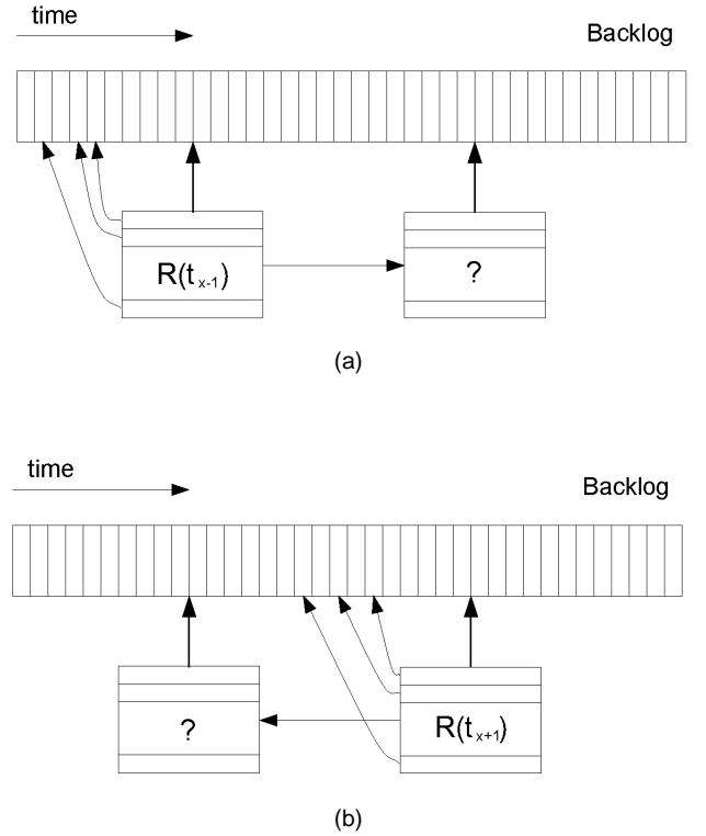
Fig. 1. Computations: (a) incremental; (b) decremental.
