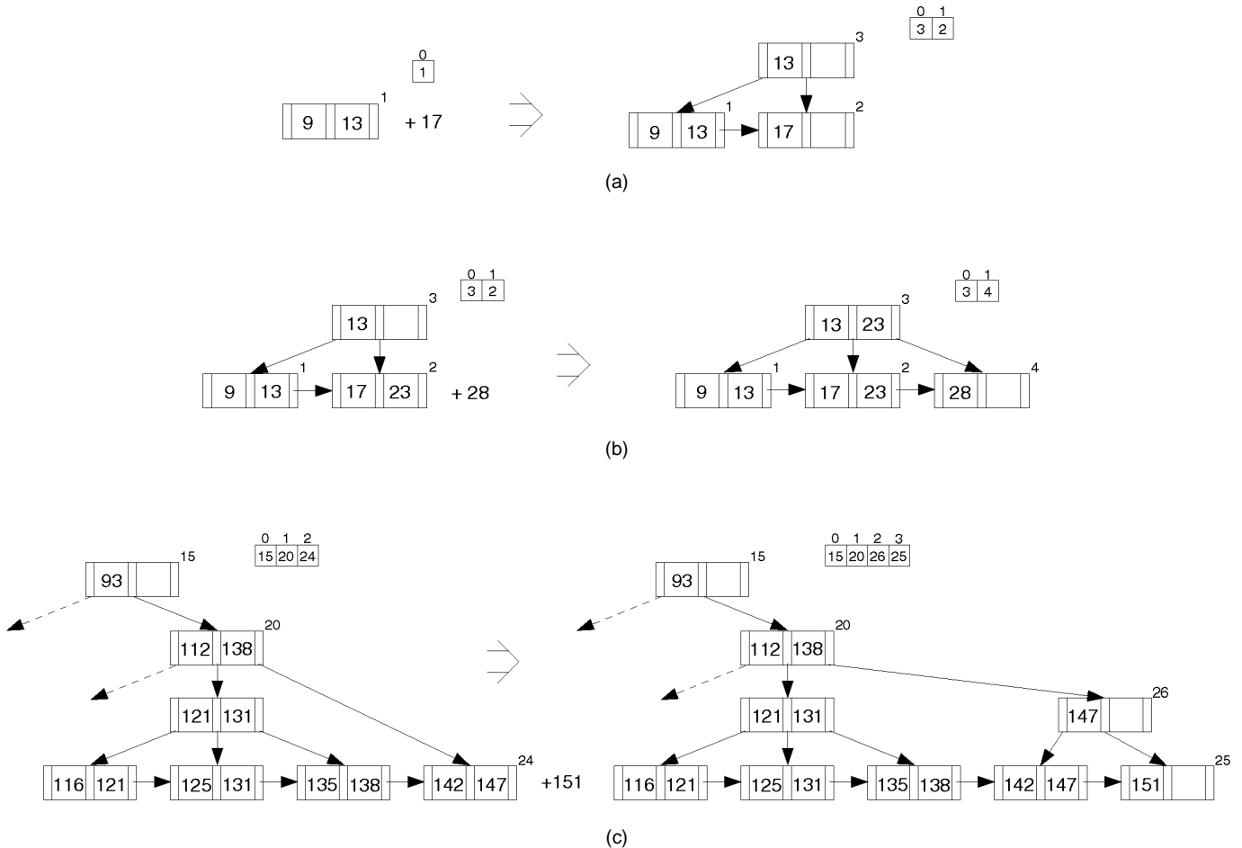
Fig. 3. Examples of insertions into the I-tree.
