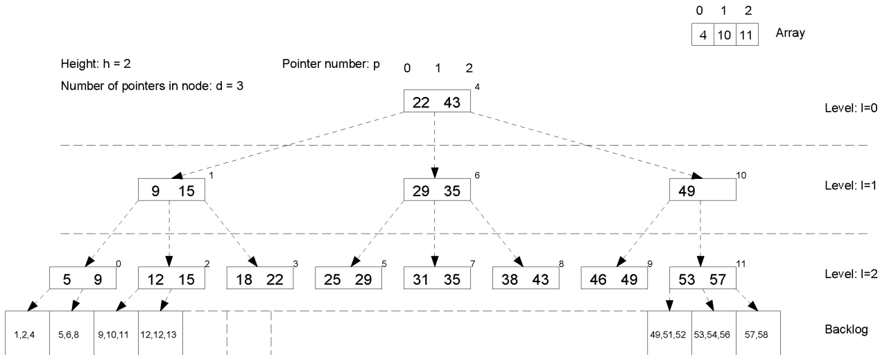
Fig. 7. A PLI-tree indexing transaction timestamps on a backlog. The pointers shown are implicit pointers.
