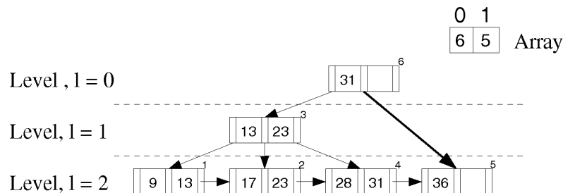
Fig. 2. An I-tree of height h = 2 and order d = 3 .
