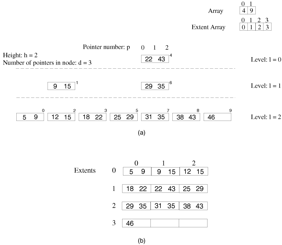
Fig. 6. An example of a PLI-tree and how nodes are stored in extents.
