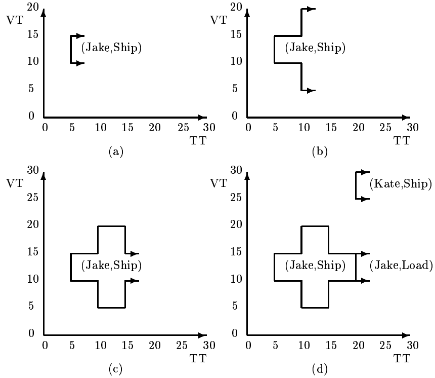
Figure 14: Bitemporal Elements
