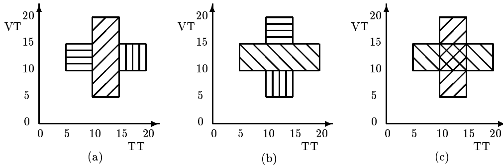
Figure 16: Example Coverings of a Bitemporal Element
