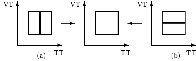
Figure 19: Coalescing
