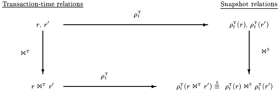
Figure 18: Reducibility of Transaction-time Natural Join to Snapshot Outer Natural Join.
