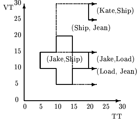
Figure 17: Graph of \text{empDep} \bowtie^B \text{mgrDep}
