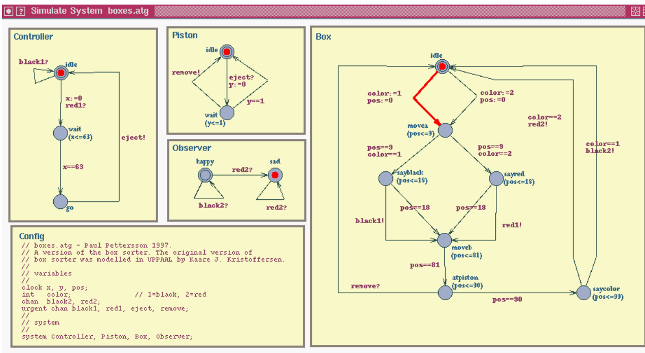
Fig. 14. A System window.
