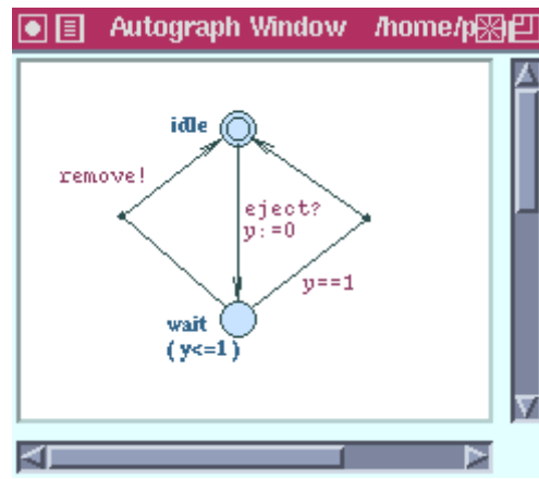
Fig. 11. Locations and transitions of the piston.
