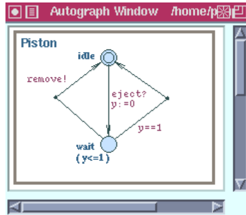
Fig. 12. An automaton defining the piston of the box-sorter unit.
