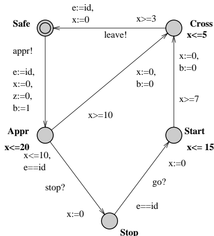
Fig. 25. The Train-Gate augmented to enable time-bounded liveness checking.
