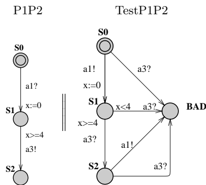
Fig. 27. A suggested abstraction and its test automaton.
