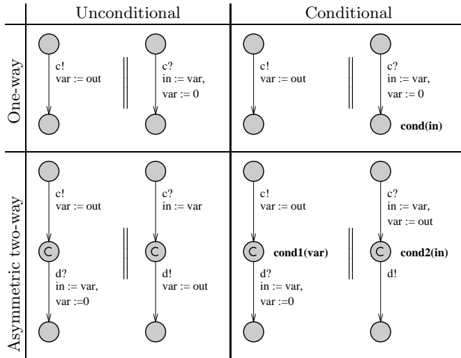
Fig. 19. There are essentially four combinations of conditional, unconditional, one-way and two-way synchronous value passing.
