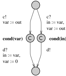
Fig. 20. In contrast to the two-way encoding shown in Fig 19, this encoding is symmetric in the sense that both automata use the exact same encoding. The symmetry comes at the cost of a slightly larger state space.
