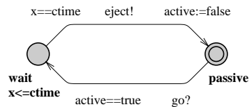
Fig. 23. Sample of a timer using an urgent edge during activation.
