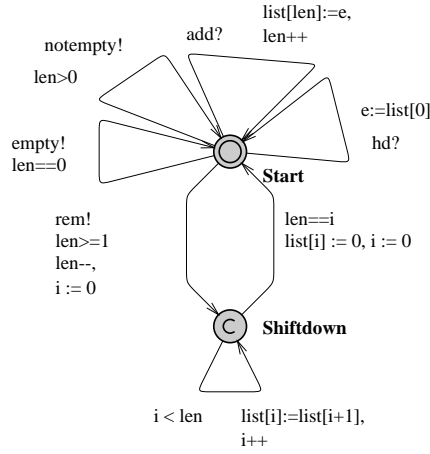
Fig. 16. Queue automaton of the train gate. The template is parameterised with int[0,n] e .
