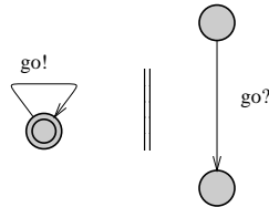
Fig. 22. Encoding of urgent edges. The go channel is declared urgent.
