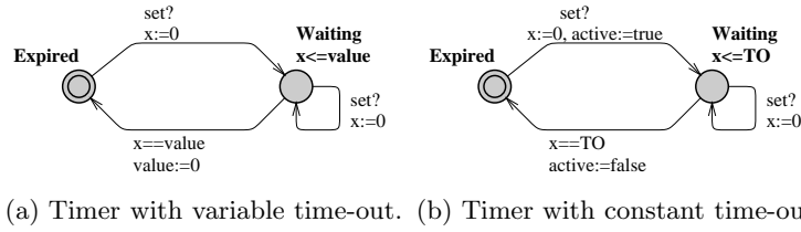
Fig. 24. Template of the timer pattern. Template (a) has int value ; chan set as parameters and template (b) has bool active ; chan set ; const T0 as parameters. Both templates have the local declaration clock x .
