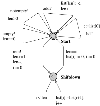
Fig. 18. The model of the queue in the train gate example uses active variable reduction twice. Both cases are on the edge from Shiftdown to Start : The freed element in the queue is reset to the initial value and so is the counter variable i .
